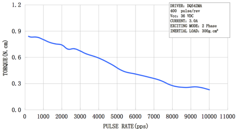
23HS6430 Torque Curve
