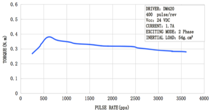
17HS4417 Torque Curve
