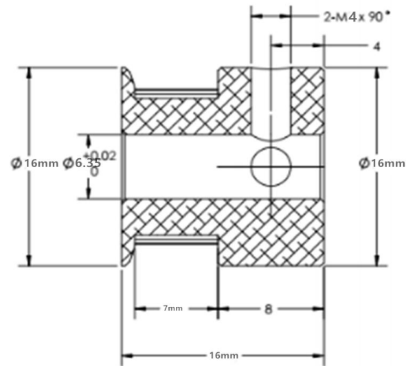
GT2 - 2mm Pitch - 20 Teeth Pulley Material: Aluminium
